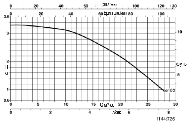
Trialine Z 65-125/034
