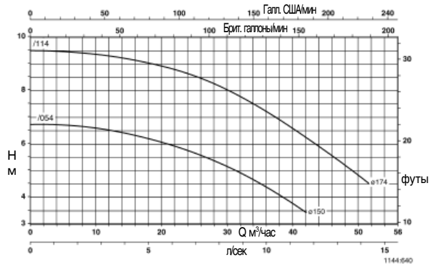
Trialine Z 50-160
