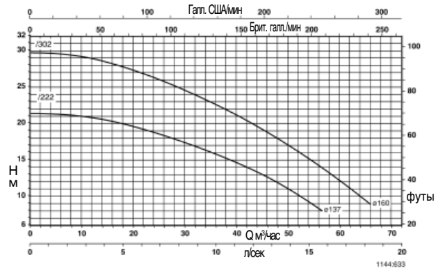
Trialine Z 40-160
