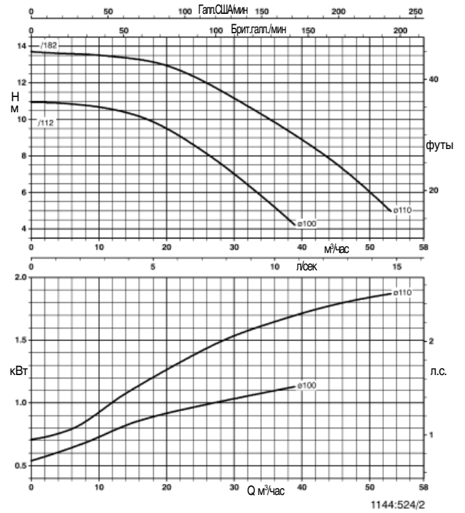
Trialine Z 65-125
