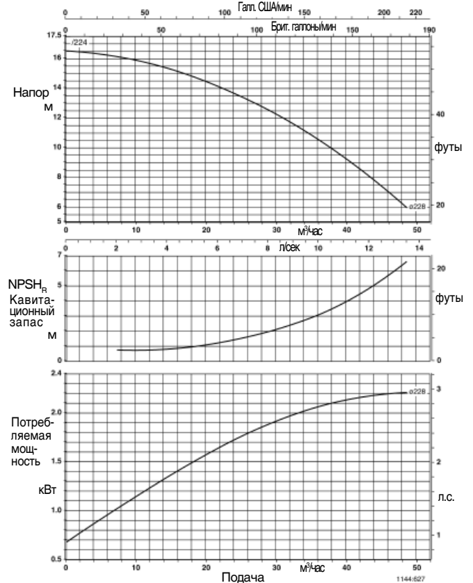
Trialine Z 50-250
