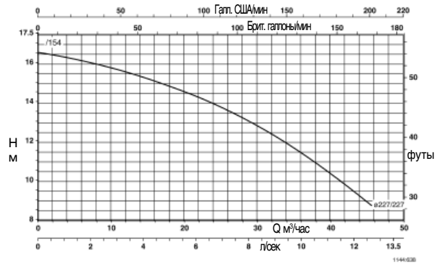
Trialine Z 40-250
