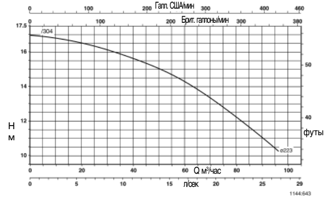
Trialine Z 65-250
