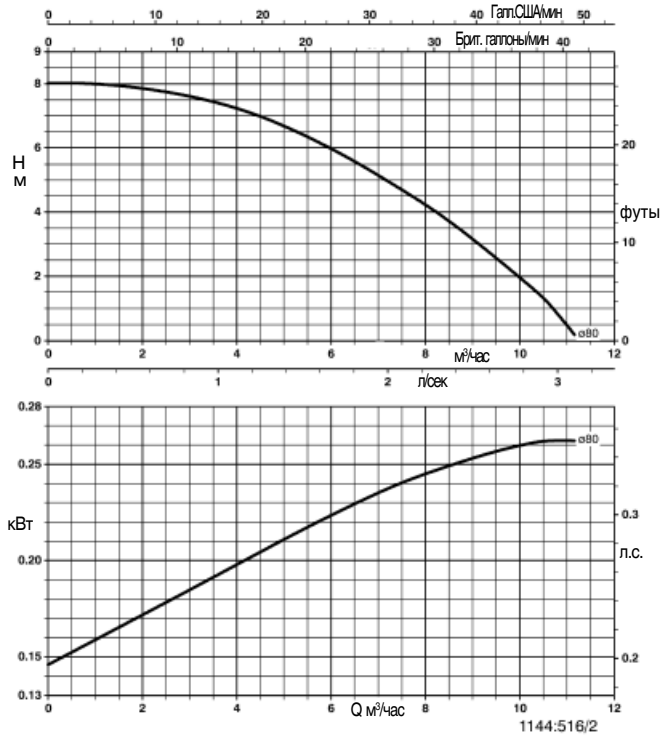
Trialine Z 32-100/022
