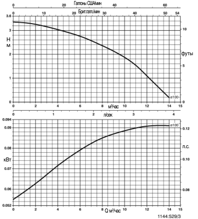
Trialine Z 40-100/014
