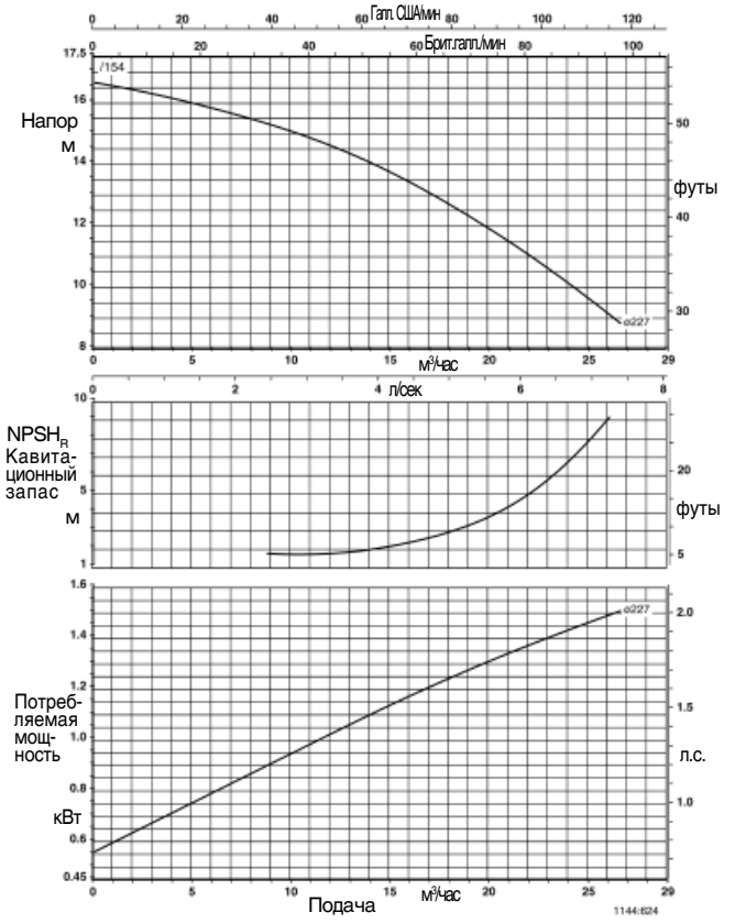
Trialine Z 50-250
