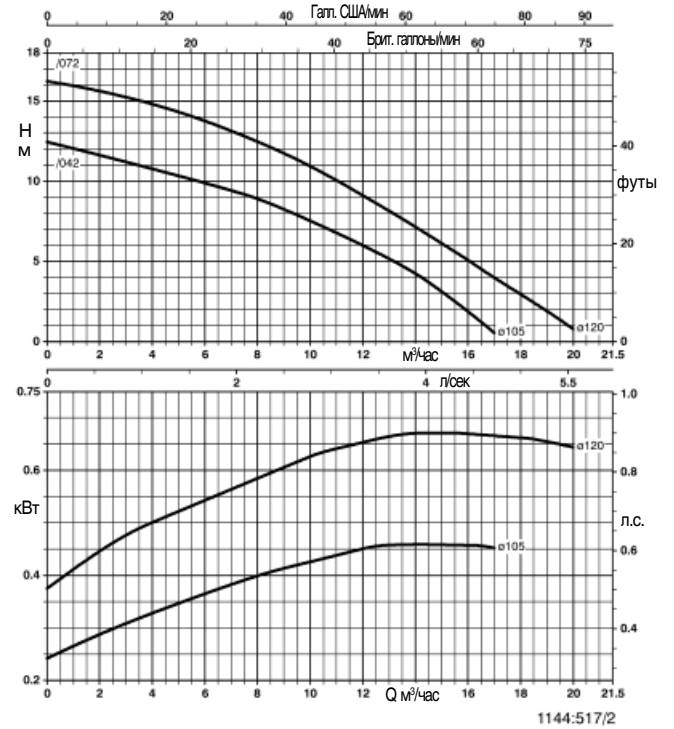
Trialine Z 32-125
