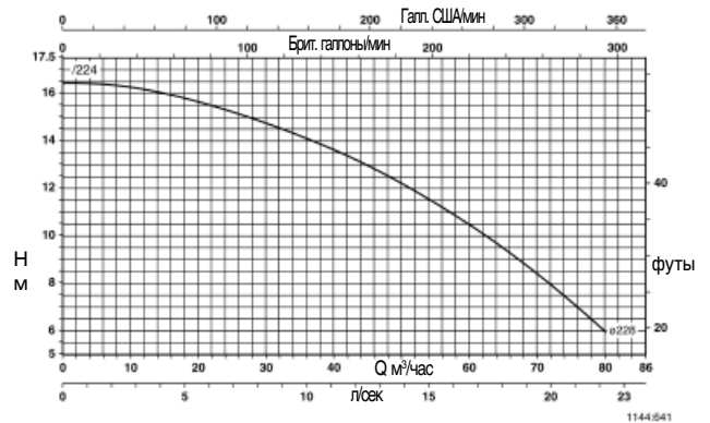
Trialine Z 50-250
